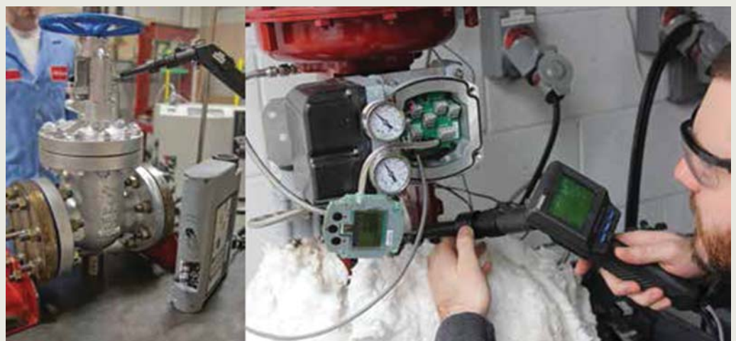
Image 1. Valve testing per ISO 15848 and API 624 (Images courtesy of Fluid Sealing Association).
